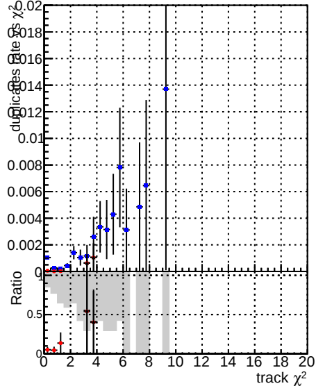
aa CMSSW mkFitPU50LowPtQuad RECO CMSSW LowPtOnoclean RECO
