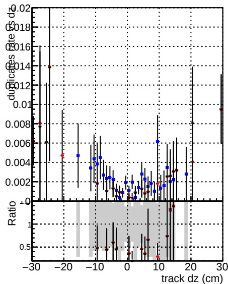
DOM V0001 R0000000001 Global CMSSW ckfPU50 RECO DOM V0001 R0000000001 Global CMSSW ckfPU50 RECO DOM V0001 R0000000001 Global CMSSW ckfPU50 RECO
