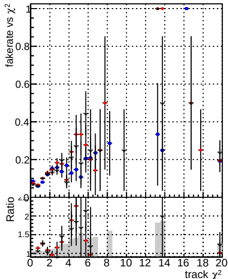
Fake rate vs. Configuration Global CMSSW ckfPU50 RECO Global CMSSW mkFitPU50LowPtQuad RECO Global CMSSW LowPtOnoclean RECO DOM V0001 Blue Red Black DOM V0001 R0000000001 Blue Red Black
