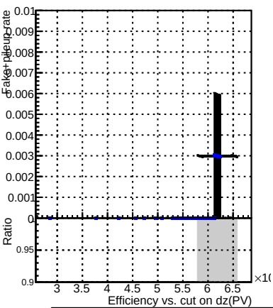
DQM_V0001_R000000001_Global_CMSSW_ckfPU50_RECO
