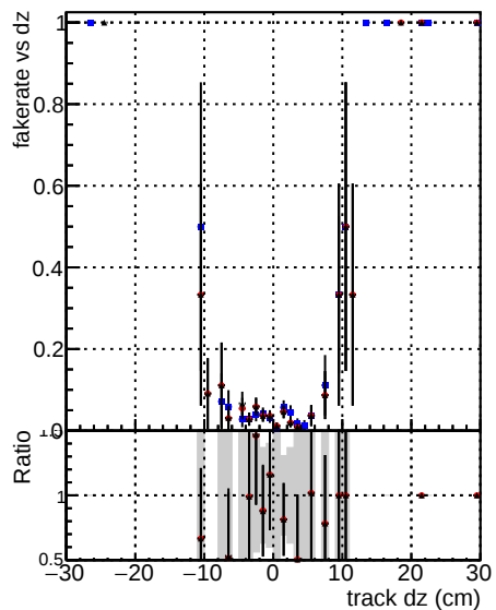
DOM_V0001 R0000000001 Global_CMSSW_ckiPU50_RECO DOM_V0001 R0000000001 Global_CMSSW_inFiPU50LowPtQuad_RECO DOM_V0001 R0000000001 Global_CMSSW_LowPtOnoclean_RECO
