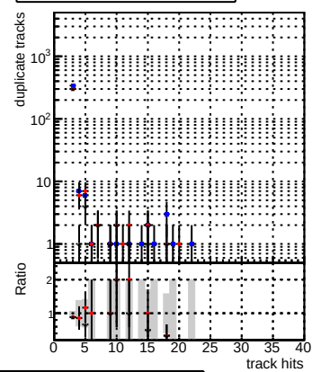
DOM V0001 R000000001 Global CMSSW ck1PU50 RECO DOM V0001 R000000001 Global CMSSW mkFitPU50LowPtQuad RECO DOM V0001 R000000001 Global CMSSW LowPtQnuclean RECO
