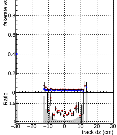
Fake rate vs dz
