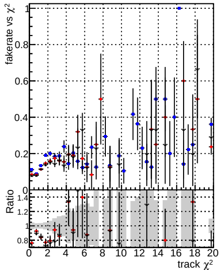
Fake rate vs. Legend DOM V0001 DOM V0001 R0000000001 Global CMSSW ckfPU50 RECO CMSSW InkFPU50LowPtQuad RECO CMSSW LowPtOnoclean RECO Line Blue Red Black Blue Red Black Point Diamond Star Dot Diamond Star Dot
