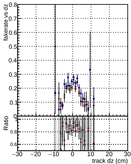
Fake rate vs d DOM V0001 R0000000001 Global CMSSW ckfPU50 RECO DOM V0001 R0000000001 Global CMSSW mkFitPU50LowPt Quad RECO DOM V0001 R0000000001 Global CMSSW LowPtNonclean RECO
