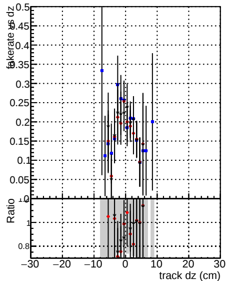
Fake rate vs dz Legend: DOM V0001 R0000000001 Global CMSSW ckfPU50 RECO DOM V0001 R0000000001 Global CMSSW InFtrPU50LowPtQuad RECO DOM V0001 R0000000001 Global CMSSW LowPtOnoclean RECO
