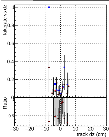
Fake rate vs d DOM V0001 R0000000001 Global CMSSW ckfPU50 RECO DOM V0001 R0000000001 Global CMSSW mkfPU50LowPt Quad RECO DOM V0001 R0000000001 Global CMSSW LowPtNonclean RECO
