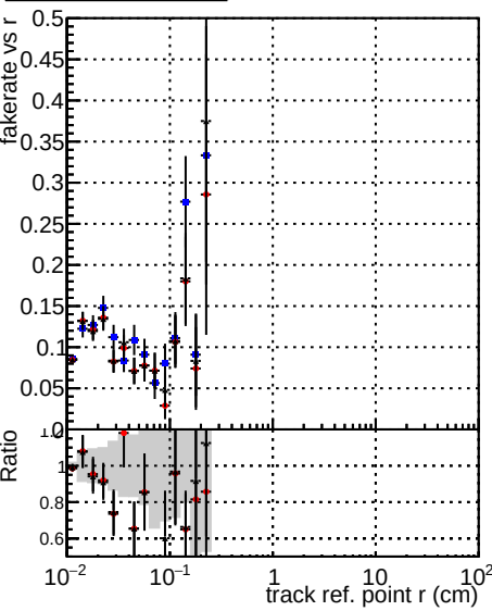
Fake rate vs verpos DQM_V0001_R000000001_Global_CMSSW_ckfPU50_RECO DQM_V0001_R000000001_Global_CMSSW_mkFitPU50LowPtQuad_RECO DQM_V0001_R000000001_Global_CMSSW_LowptQnoclean_RECO
