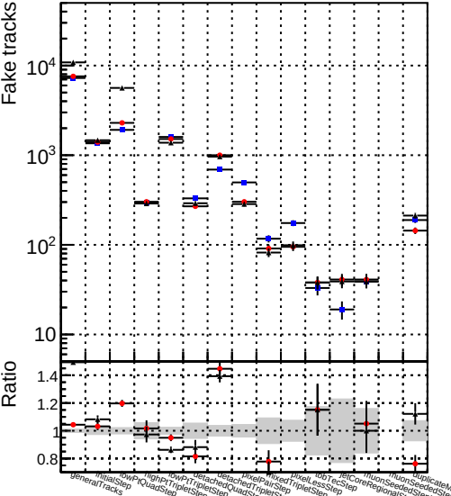
Number Legend Dataset Model Task DQM_V0001_R0000000001 Global CMSSW_ckfPU50_RECO DQM_V0001_R0000000001 Global CMSSW_mkFitPU50_LowPtQuad_RECO DQM_V0001_R0000000001 Global CMSSW_LowptQnoclean_RECO
