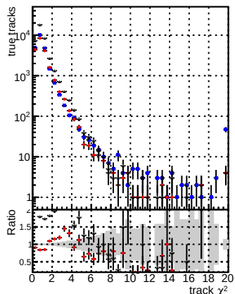
N of reco track vs. \chi^2 for Global CMSSW v0001 (blue circles), Global CMSSW v0001 (red circles), and Global CMSSW v0001 (black circles). The legend also includes Global CMSSW v0001 (grey circles) and Global CMSSW v0001 (white circles).
