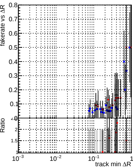
Fake rate vs \Delta R(\text{track, jet}) Legend: DQM_V0001_R000000001_Global_CMSSW_ckfPU50_RECO (blue dots) DQM_V0001_R000000001_Global_CMSSW_mkFitPU50LowPtQuad_RECO (red dots) DQM_V0001_R000000001_Global_CMSSW_LowptQnoclean_RECO (black dots)
