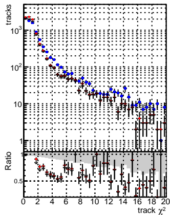
N of reco track vs. s DQM V0001 R00000000001 Global CMSSW_KIT_030 RECO DQM V0001 R00000000001 Global mkFitPU50LowPtQuad RECO DQM V0001 R00000000001 Global LowPtQnClean RECO DQM V0001 R00000000001 Global LowPtQnClean RECO
