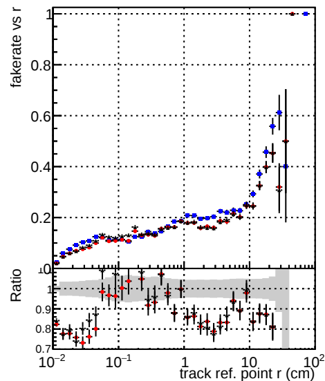
—●— DQM_V0001_R000000001 Global CMSSW ckfPU50 RECO —●— DQM_V0001_R000000001 Global CMSSW mkFitPU50LowPtQuad RECO —+— DQM_V0001_R000000001 Global CMSSW LowptQnoclean RECO
