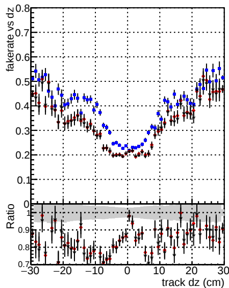
DOM V0001 R0000000001 Global CMSSW ckfPU50 RECO DOM V0001 R0000000001 Global CMSSW InkFIRPU50 LowPtQuad_RECO DOM V0001 R0000000001 Global CMSSW LowPtOnoclean RECO
