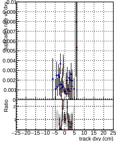
DOM V0001 R0000000001 Global CMSSW ckfPU50 RECO DOM V0001 R0000000001 Global CMSSW InkFIRPU50 LowPtQuad_RECO DOM V0001 R0000000001 Global CMSSW LowPtOnoclean RECO
