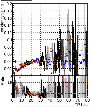
Efficiency vs hit Legend: DQM_V0001_R000000001_Global_CMSSW_ckf_RECO DQM_V0001_R000000001_Global_CMSSW_mkFitOriginal_RECO DQM_V0001_R000000001_Global_CMSSW_mkFitLowPtQuad_RECO DQM_V0001_R000000001_Global_CMSSW_mkFitLowPtTriplet_RECO
