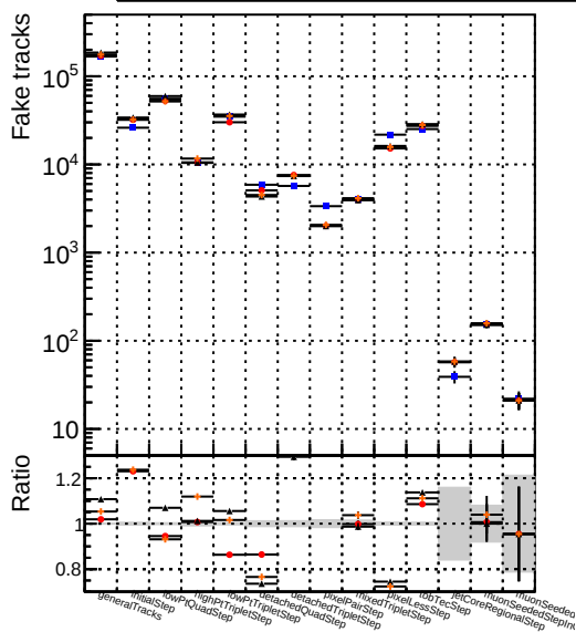
Number ■ DQM_V0001 R000000001 Global CMSSW_ckpt_RECO ■ DQM_V0001 R000000001 Global CMSSW_mkFitOriginal_RECO ■ DQM_V0001 R000000001 Global CMSSW_mkFitLowPtQuad_RECO ■ DQM_V0001 R000000001 Global CMSSW_mkFitLowPtTriplet_RECO
