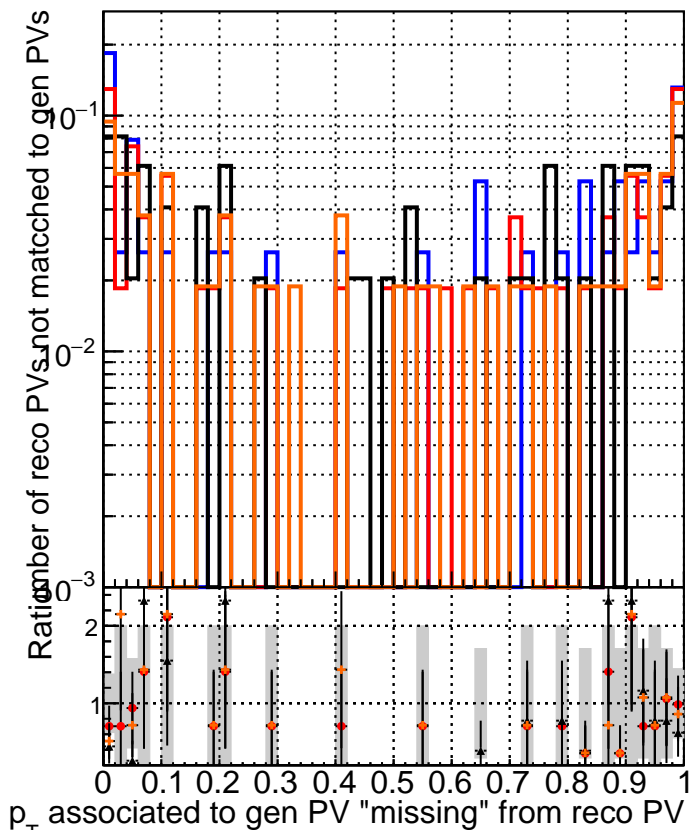
RecoPVAssoc2GenPVNotMatched_missing
