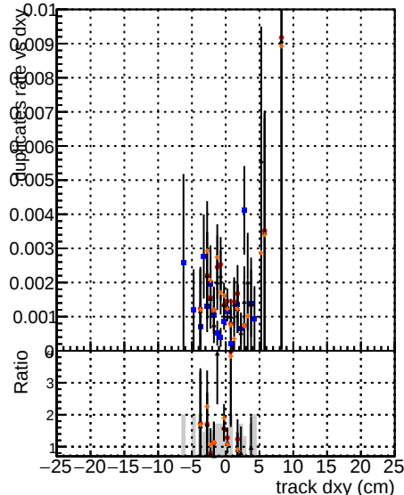
LOW Quad RECO LOW Triplet RECO
