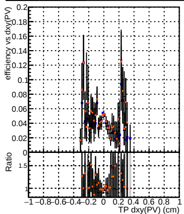
Efficiency DQM_V0001_R0000000001_Global_CMSSW_ckf_RECO DQM_V0001_R0000000001_Global_CMSSW_mkFitOriginal_RECO DQM_V0001_R0000000001_Global_CMSSW_mkFitLowPtQuad_RECO DQM_V0001_R0000000001_Global_CMSSW_mkFitLowPtTriplet_RECO
