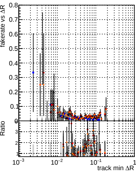
Fake rate vs \Delta R(\text{track, jet}) Legend: Global CMSSW mktFit RECO Global CMSSW mktFit Original RECO Global CMSSW mktFit LowPtTriplet RECO
