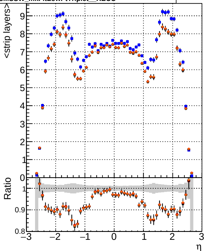
Legend: ■ DQM_V0001_R0000000001 Global CMSSW_ckf_RECO ● DQM_V0001_R0000000001 Global CMSSW_mkFitOriginal_RECO ▲ DQM_V0001_R0000000001 Global CMSSW_mkFitLowPtQuad_RECO ◆ DQM_V0001_R0000000001 Global CMSSW_mkFitLowPtTriplet_RECO
