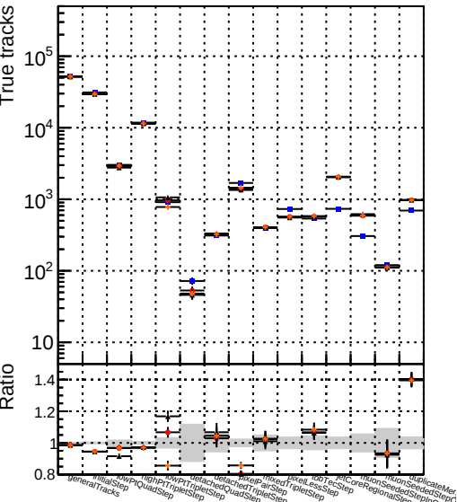
Number Color Model Fit Type Fit Order Fit Name 1 Blue DOM V0001 R0000000001 Global CMSSW_ckt_REC0 2 Red DOM V0001 R0000000001 Global CMSSW_mkFitOriginal_REC0 3 Green DOM V0001 R0000000001 Global CMSSW_mkFitLowPtQuad_REC0 4 Orange DOM V0001 R0000000001 Global CMSSW_mkFitLowPtTriplet_REC0
