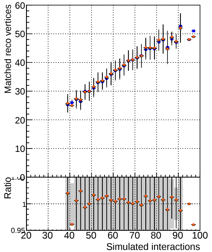
MatchedRecoVtx_vs_GenVtx
