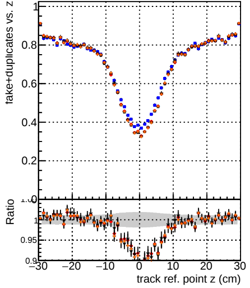
—●— DQM_V0001_R0000000001_Global_CMSSW_ckpt_RECO —●— DQM_V0001_R0000000001_Global_CMSSW_mkFitOriginal_RECO —●— DQM_V0001_R0000000001_Global_CMSSW_mkFitLowPtQuad_RECO —●— DQM_V0001_R0000000001_Global_CMSSW_mkFitLowPtTriplet_RECO
