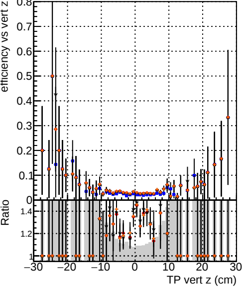
—●— DQM_V0001_R0000000001_Global_CMSSW_ckpt_RECO —●— DQM_V0001_R0000000001_Global_CMSSW_mkFitOriginal_RECO —●— DQM_V0001_R0000000001_Global_CMSSW_mkFitLowPtQuad_RECO —●— DQM_V0001_R0000000001_Global_CMSSW_mkFitLowPtTriplet_RECO
