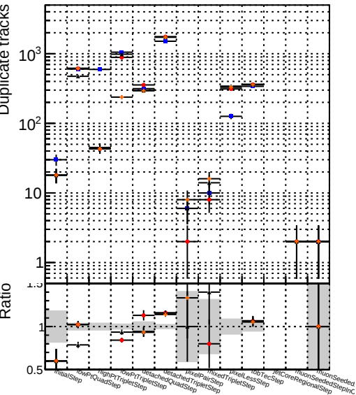
Number Model Fit Model Fit Model Fit Model Fit 1 DQM V0001 R0000000001 Global CMSSW ckf RECO 2 DQM V0001 R0000000001 Global CMSSW mkFit Original RECO 3 DQM V0001 R0000000001 Global CMSSW mkFit LowPQuad RECO 4 DQM V0001 R0000000001 Global CMSSW mkFit LowPTriplet RECO
