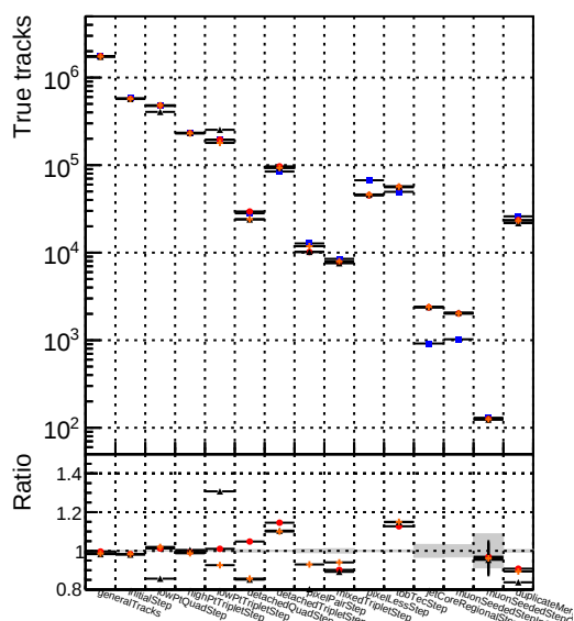
Number Legend DQM V0001 R000000001 Global CMSSW ckf RECO ● DQM V0001 R000000001 Global CMSSW mkFitOriginal RECO ● DQM V0001 R000000001 Global CMSSW mkFitLowPtQuad RECO ● DQM V0001 R000000001 Global CMSSW mkFitLowPtTriplet RECO
