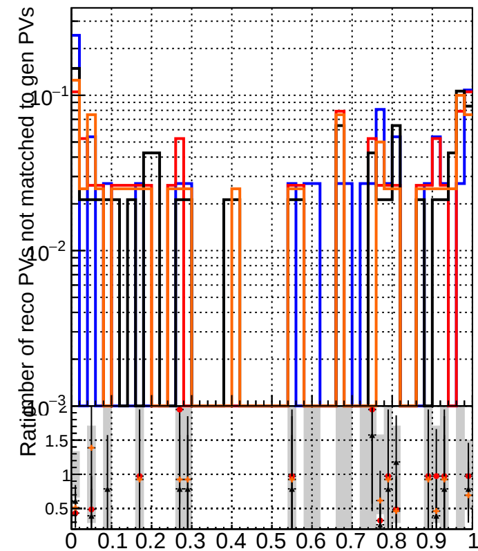
RecoPVAssoc2GenPVnotmatched_missing
