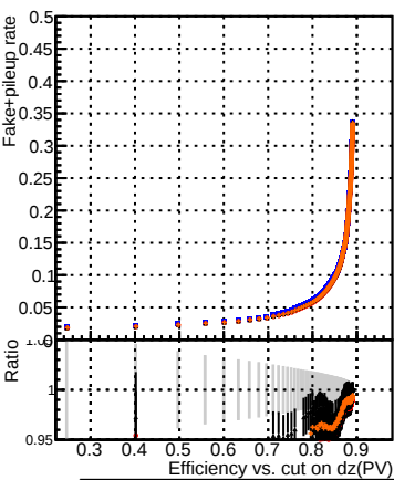
Efficiency vs. cut on dz(PV) —●— DQM_V0001_R000000001_Global_CMSSW_ckfPU50_RECO —●— DQM_V0001_R000000001_Global_CMSSW_mkFitPU50LowPtQuad_RECO —●— DQM_V0001_R000000001_Global_CMSSW_LowptQnoclean_RECO —●— DQM_V0001_R000000001_Global_CMSSW_looseSC_RECO
