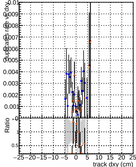
CMSSW-LowPtoClean RECO
