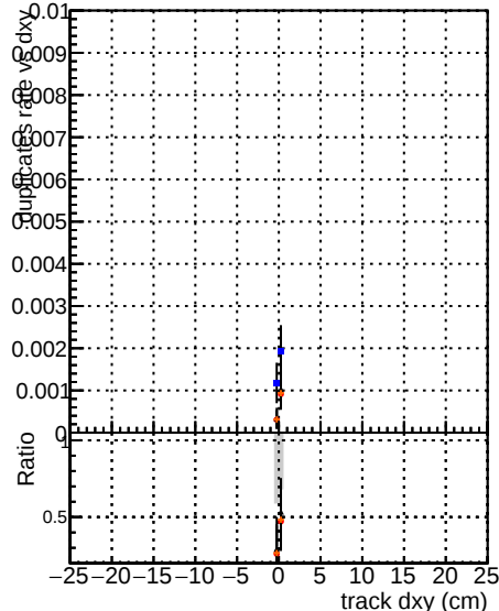
CMSSW-LowPtoNoclean RECO CMSSW-looseSC RECO
