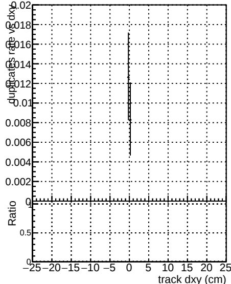
CMSSW-LowPtoClean RECO
