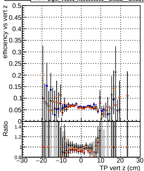
—●— DQM_V0001_R000000001_Global_CMSSW_cktPU50_RECO —◆— DQM_V0001_R000000001_Global_CMSSW_mkFitPU50LowPtQuad_RECO —★— DQM_V0001_R000000001_Global_CMSSW_LowptQnoclean_RECO —×— DQM_V0001_R000000001_Global_CMSSW_looseSC_RECO
