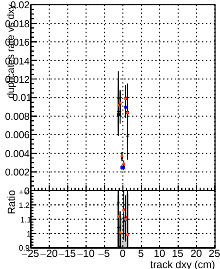
CMSSW LooseSC REC
