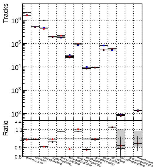
—●— DQM_V0001_R000000001_Global_CMSSW_ckfPU50_RECO —●— DQM_V0001_R000000001_Global_CMSSW_mkFitPU50LowPtQuad_RECO —●— DQM_V0001_R000000001_Global_CMSSW_LowPtQnoclean_RECO
