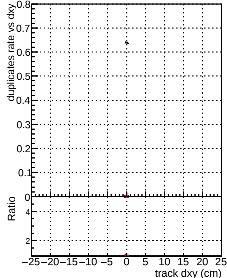
—CMSSW—mkFitPU50LowPtQuad—RECO —CMSSW—LowPtOnoclean—RECO
