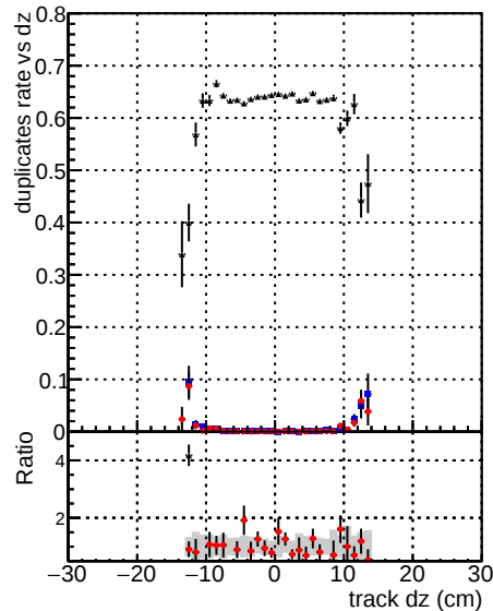
—CMSSW—mkFitPU50LowPtQuad—RECO —CMSSW—LowPtOnoclean—RECO
