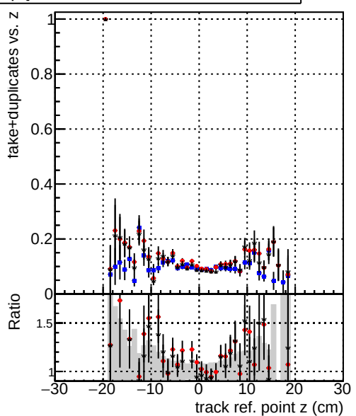
—●— DQM_V0001_R0000000001_Global_CMSSW_ckFitPU50_RECO —●— DQM_V0001_R0000000001_Global_CMSSW_mkFitPU50LowPtQuad_RECO —●— DQM_V0001_R0000000001_Global_CMSSW_LowptQnoclean_RECO
