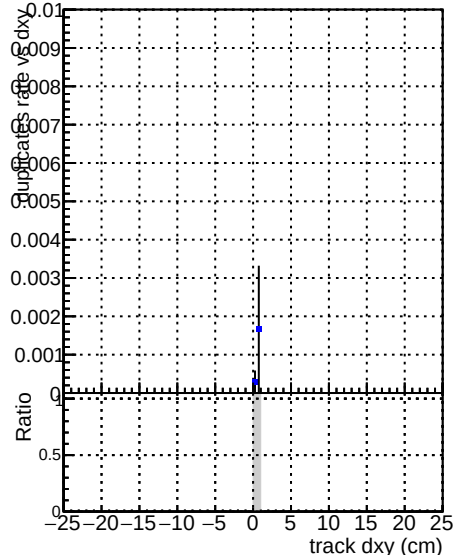
Model CMSSW mkFit PU50 LowPt Quad RECO all CMSSW LowPt Onoclean RECO
