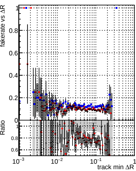
Fake rate vs \Delta R(\text{track, jet}) Legend: DQM_V0001_R000000001_Global_CMSSW_ckfPU50_RECO DQM_V0001_R000000001_Global_CMSSW_mkFitPU50LowPtQuad_RECO DQM_V0001_R000000001_Global_CMSSW_LowptQnoclean_RECO
