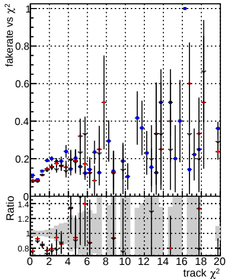
Fake rate vs. DOM V0001 R0000000001 Global CMSSW ckfPU50 RECO DOM V0001 R0000000001 Global CMSSW mkFPU50LowPtQuad RECO DOM V0001 R0000000001 Global CMSSW LowPtOnoclean RECO
