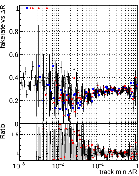
Fake rate vs \Delta R(\text{track, jet}) Duplicates Rate vs \Delta R(\text{track, jet}) Pileup rate vs \Delta R(\text{track, jet}) Legend: DQM_V0001_R000000001 Global CMSSW_ckfPU50_RECO DQM_V0001_R000000001 Global CMSSW_mkFitPU50LowPtQuad_RECO DQM_V0001_R000000001 Global CMSSW_LowPtQnoclean_RECO
