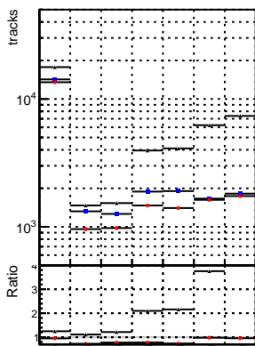
N of reco track vs. s DQM V0001 R0000000001 Global CMSSW CRFPU50-RECO DQM V0001 R0000000001 Global CMSSW mkFitPU50LowPtQuad RECO DQM V0001 R0000000001 Global CMSSW LowPtQnuclear RECO
