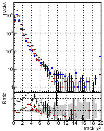
N of reco track vs. s DQM V0001 R0000000001 Global CMSSW CRFPU50-RECO DQM V0001 R0000000001 Global CMSSW mkFitPU50LowPtQuad RECO DQM V0001 R0000000001 Global CMSSW LowPtQnuclear RECO
