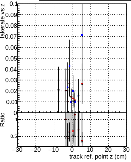
Legend: - Global CMSSW ckfPU50 RECO - Global CMSSW mkFitPU50LowPtQuad RECO - Global CMSSW LowptQnoclean RECO
