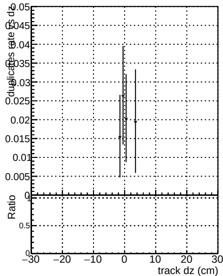
a CMSSW mkFitPU50Low a CMSSW LowptOnoclea
