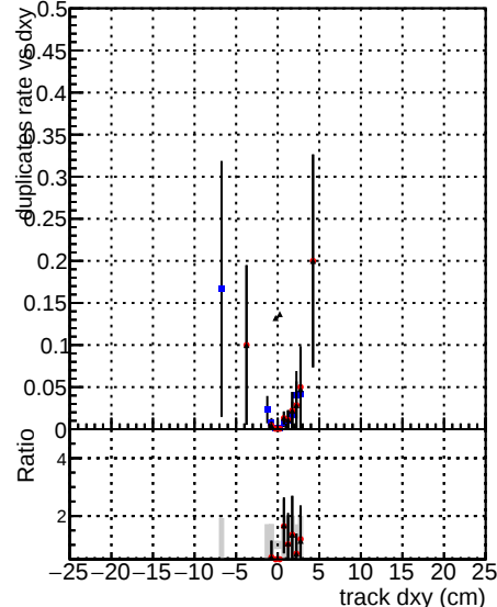
DOM V0001 R0000000001 Global CMSSW ckfPU50 RECO DOM V0001 R0000000001 Global CMSSW InFtPU50 LowPtQuad RECO DOM V0001 R0000000001 Global CMSSW LowPtOnClean RECO
