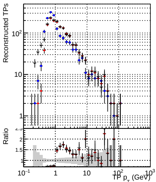
● DQM_V0001_R000000001_Global_CMSSW_ckfPU50_RECO ● DQM_V0001_R000000001_Global_CMSSW_mkFitPU50LowPtQuad_RECO ● DQM_V0001_R000000001_Global_CMSSW_LowptQnoclean_RECO
