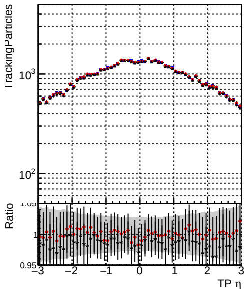
● DQM_V0001_R000000001_Global_CMSSW_ckfPU50_RECO ● DQM_V0001_R000000001_Global_CMSSW_mkFitPU50LowPtQuad_RECO ● DQM_V0001_R000000001_Global_CMSSW_LowptQnoclean_RECO
