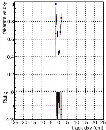
DOM V0001 R0000000001 Global CMSSW ckPU50 RECO DOM V0001 R0000000001 Global CMSSW InFIRPU50LowPtQuad RECO DOM V0001 R0000000001 Global CMSSW LowPtQuadClean RECO
